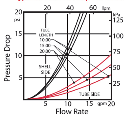
Typical Pressure Drop For Water
