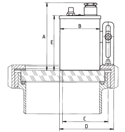
Types BKVLR 20 / 50 H(D)Sch1 Type BKVLR 100 HDSch1
