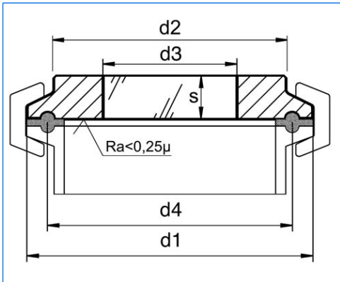
Typical assembly
